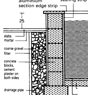
8 Masonry pool with drainage
